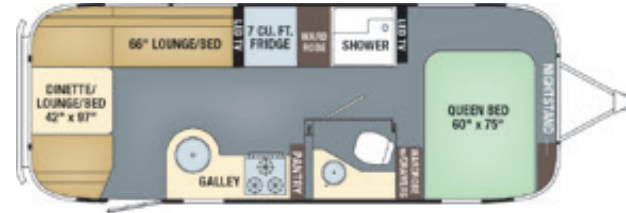
25FB
